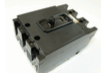
Siemens EE3B020 3p 20a 240v Circuit Breaker / ITE / Gould Molded Case (used) Siemens EE3B020 3p 20a 240v Circuit Breaker / ITE / Gould Molded Case (used)
